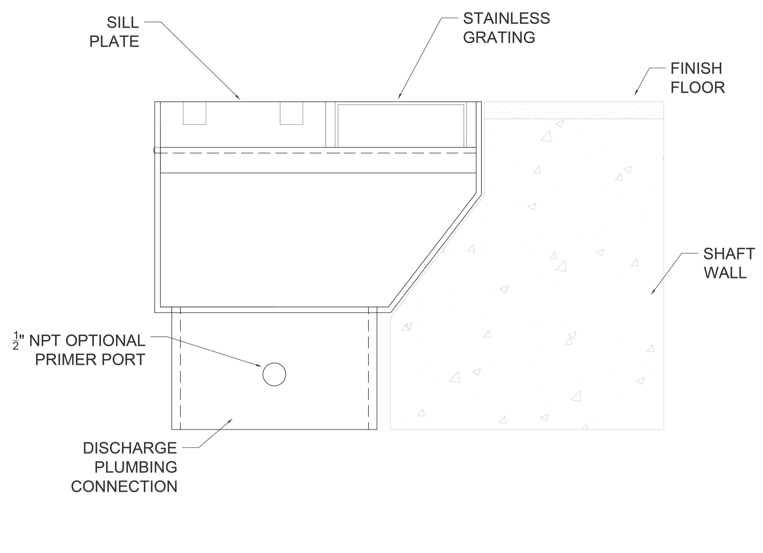
SILL PLATE DETAIL SCALE: 1"-1"
